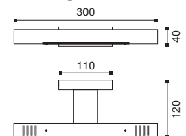
attacco parete wall fixing
