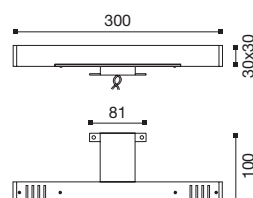
attacco piastra plate fixing
